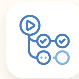
GITHUB ACTIONS
